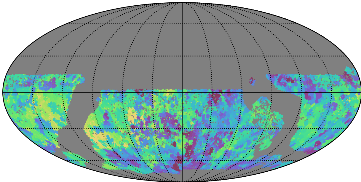
baseline_v3.0_10yrs WFD r band: Min saturation_mag
