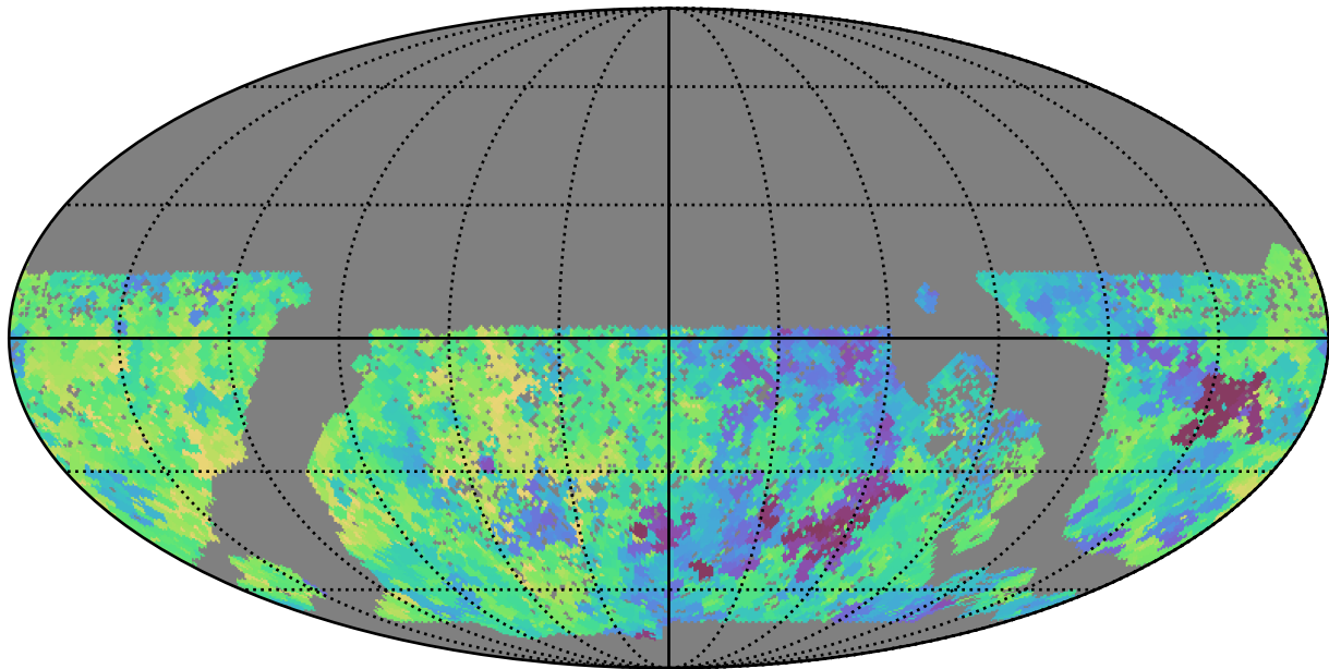
baseline_v3.0_10yrs WFD i band: Min saturation_mag
