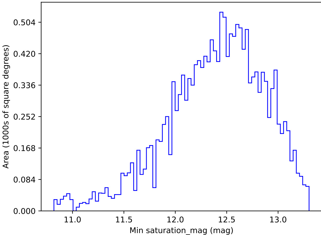
baseline_v3.0_10yrs WFD i band: Min saturation_mag
