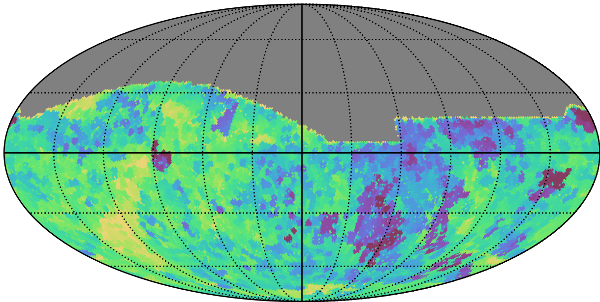
baseline_v3.0_10yrs All sky z band: Min saturation_mag
