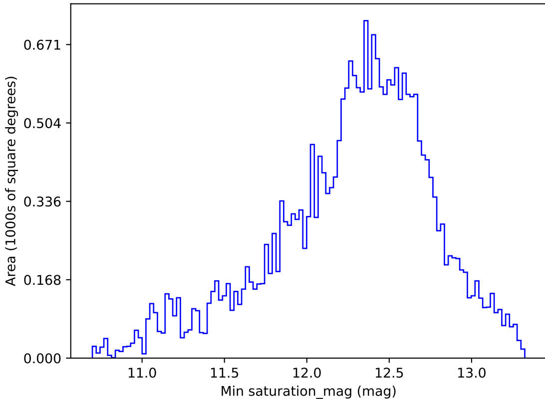
baseline_v3.0_10yrs All sky z band: Min saturation_mag
