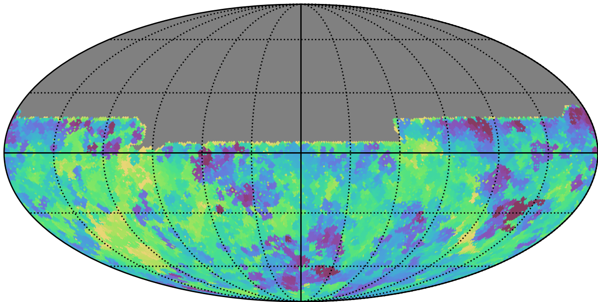
baseline_v3.0_10yrs All sky u band: Min saturation_mag
