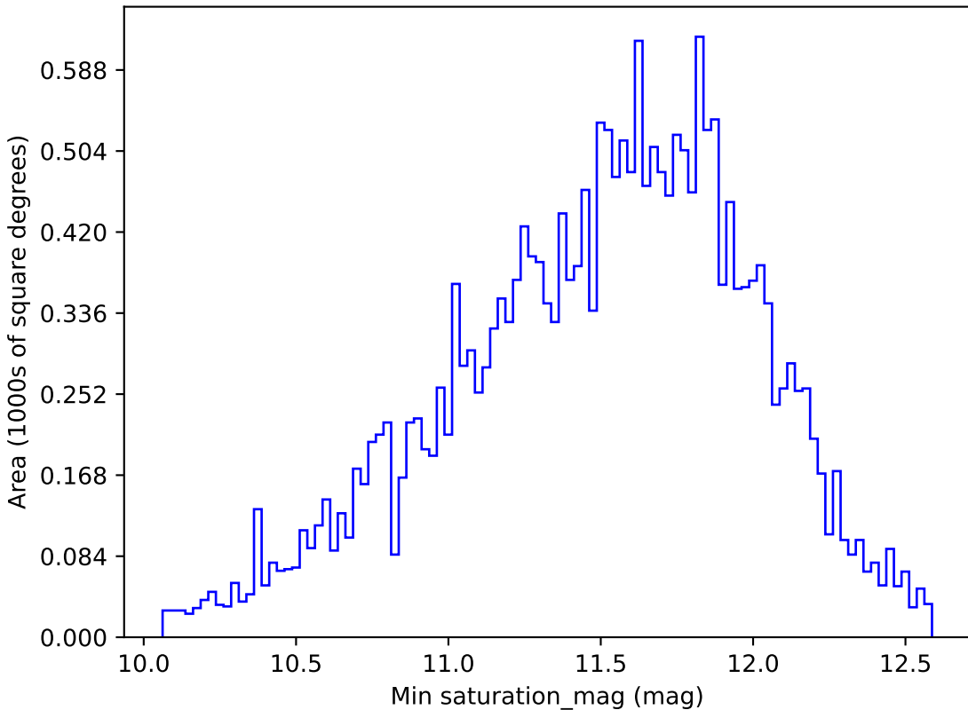
baseline_v3.0_10yrs All sky u band: Min saturation_mag
