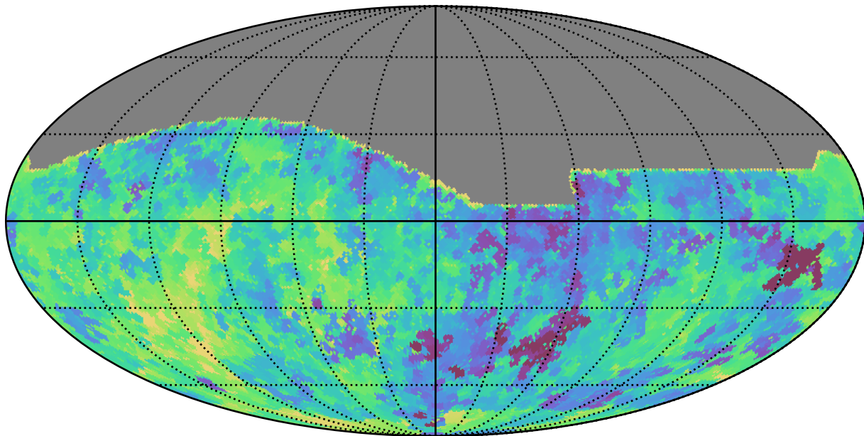
baseline_v3.0_10yrs All sky i band: Min saturation_mag
