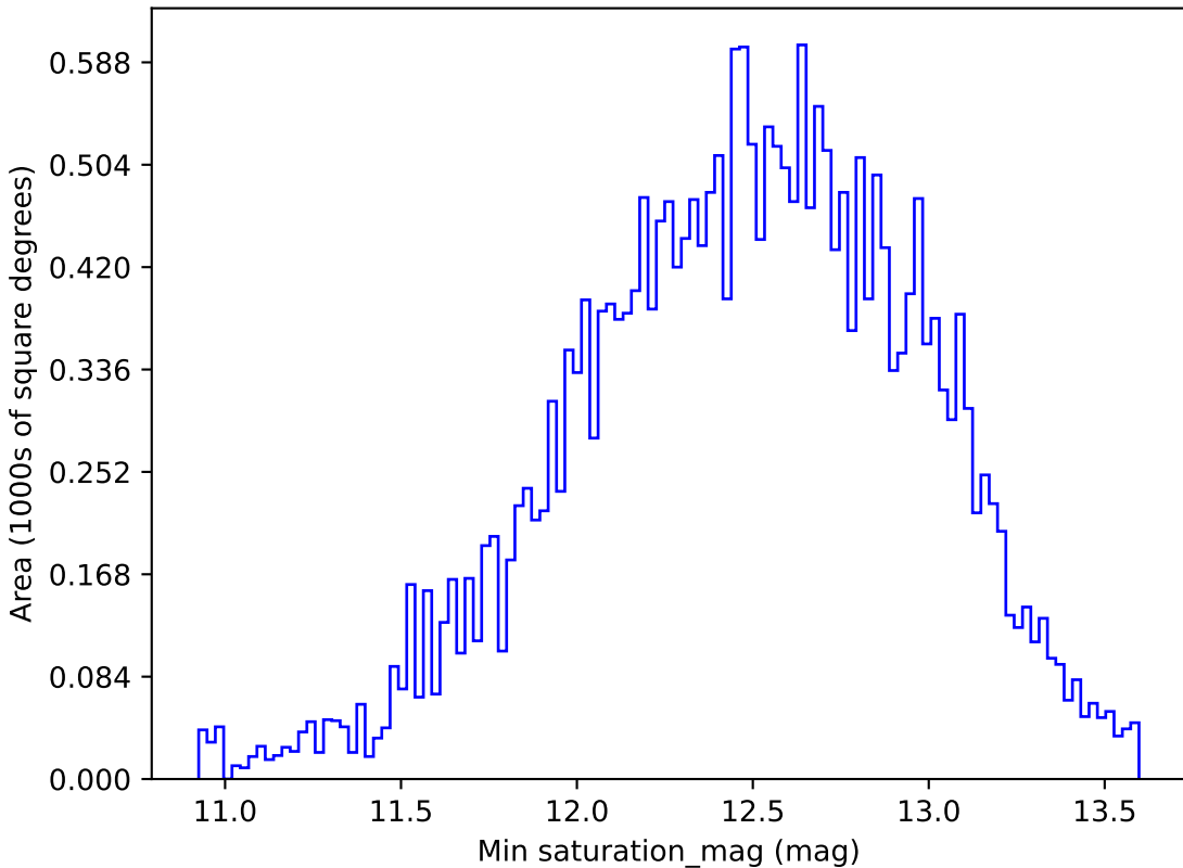
baseline_v3.0_10yrs All sky i band: Min saturation_mag
