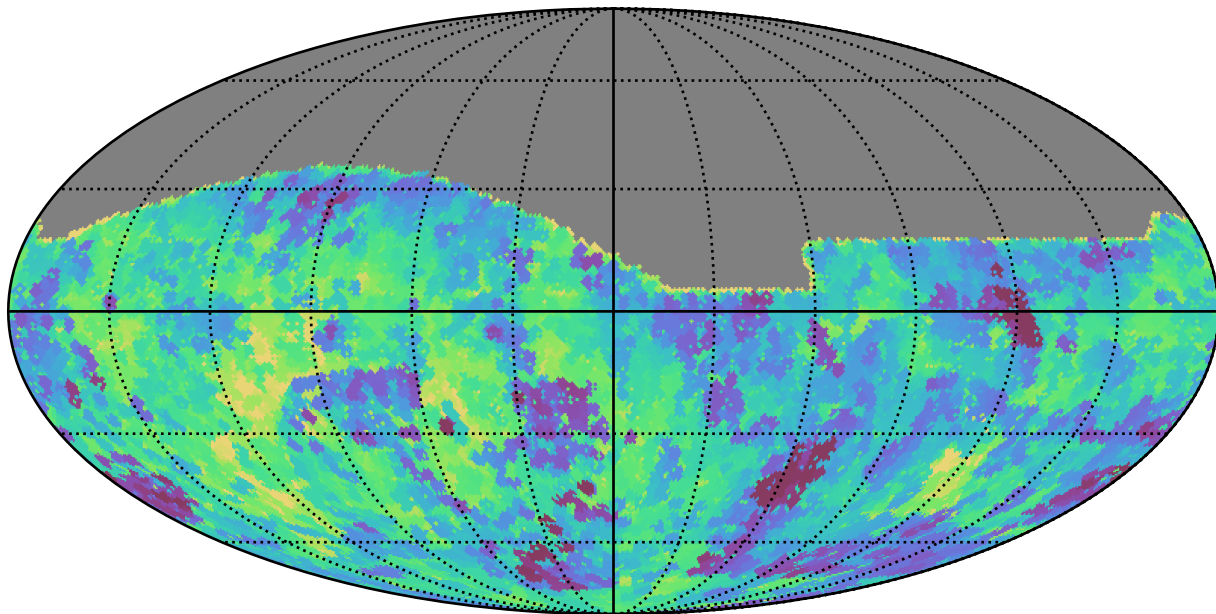
baseline_v3.0_10yrs All sky g band: Min saturation_mag
