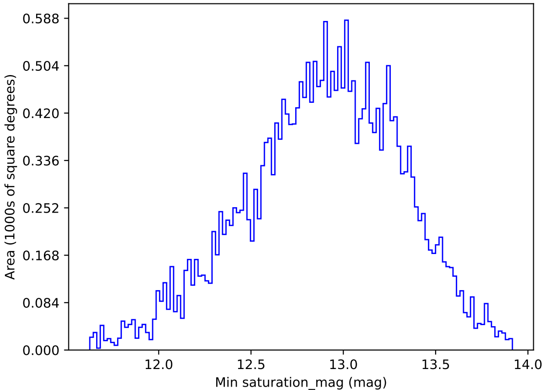
baseline_v3.0_10yrs All sky g band: Min saturation_mag
