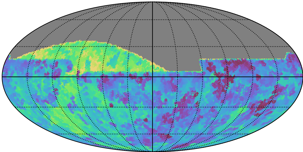
baseline_v3.0_10yrs All sky all bands: Min saturation_mag
