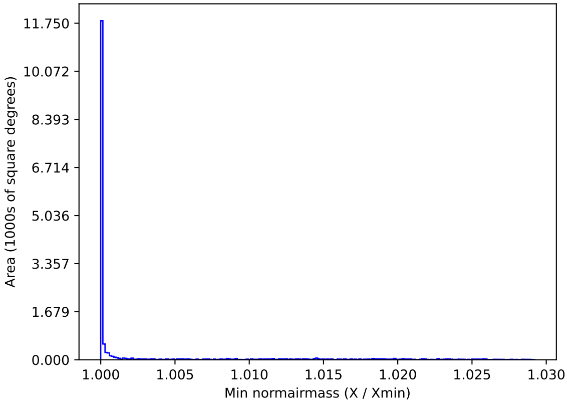
baseline_v3.0_10yrs WFD z band: Min normairmass
