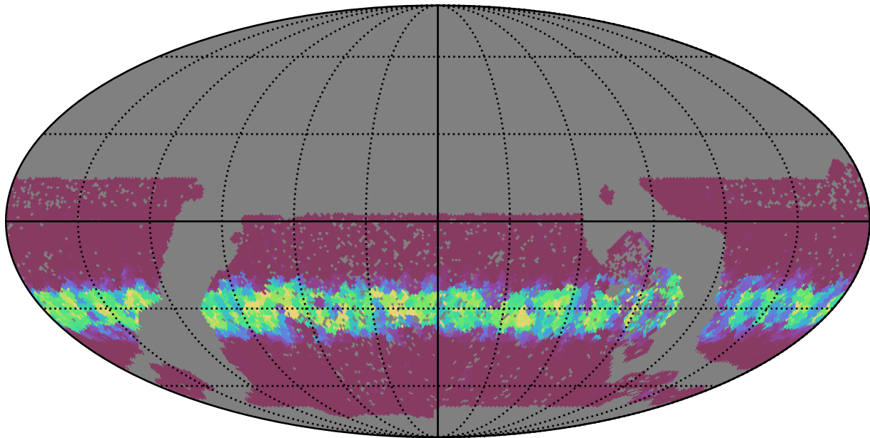
baseline_v3.0_10yrs WFD u band: Min normairmass
