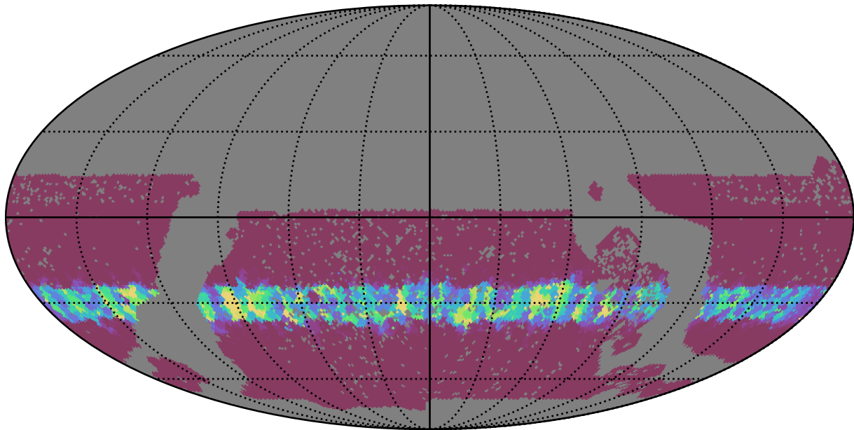
baseline_v3.0_10yrs WFD r band: Min normairmass
