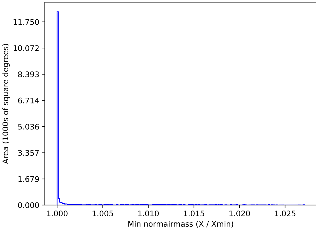
baseline_v3.0_10yrs WFD i band: Min normairmass
