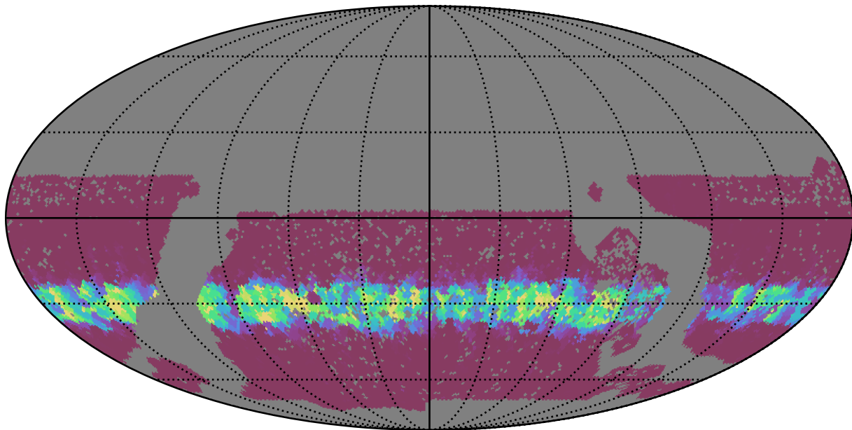
baseline_v3.0_10yrs WFD g band: Min normairmass
