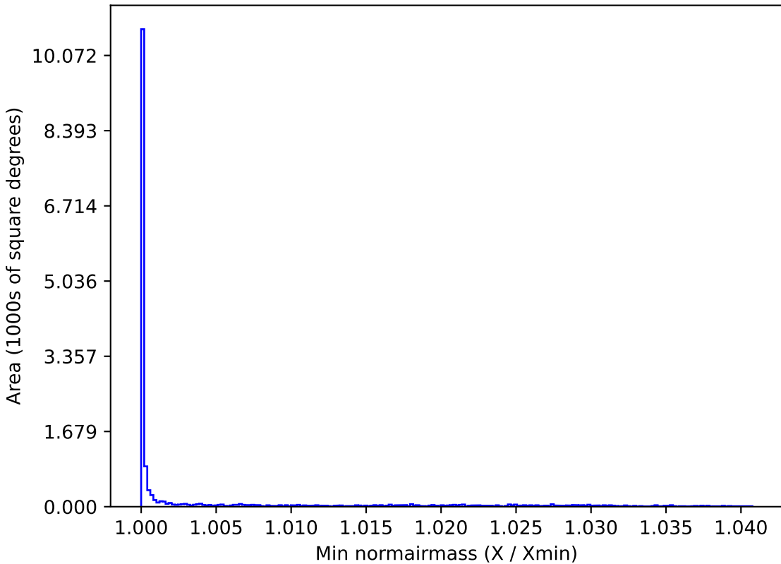
baseline_v3.0_10yrs WFD g band: Min normairmass
