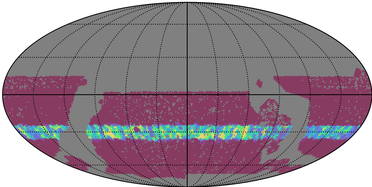
baseline_v3.0_10yrs WFD all bands: Min normairmass
