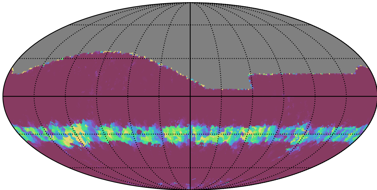
baseline_v3.0_10yrs All sky z band: Min normairmass
