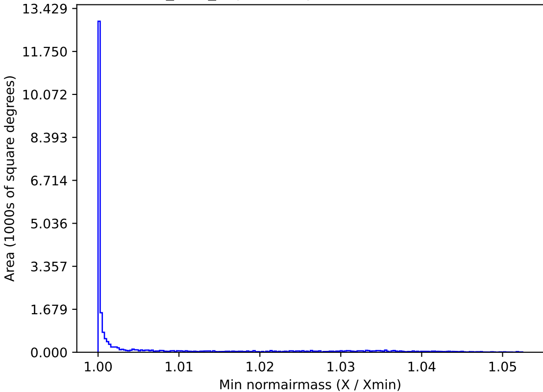
baseline_v3.0_10yrs All sky u band: Min normairmass
