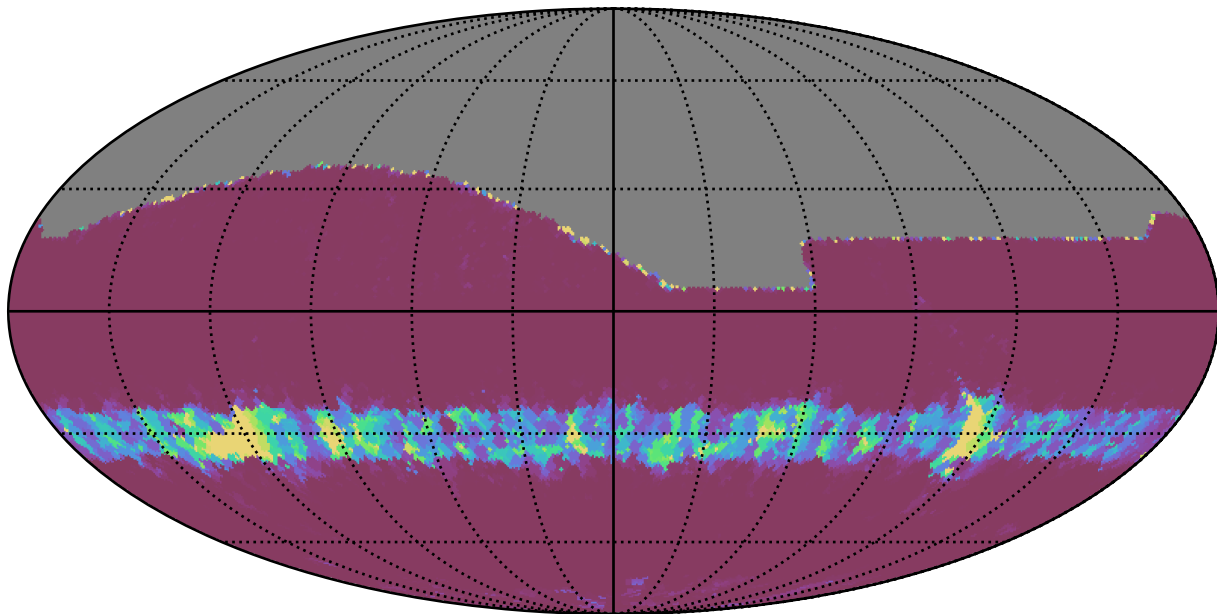
baseline_v3.0_10yrs All sky r band: Min normairmass
