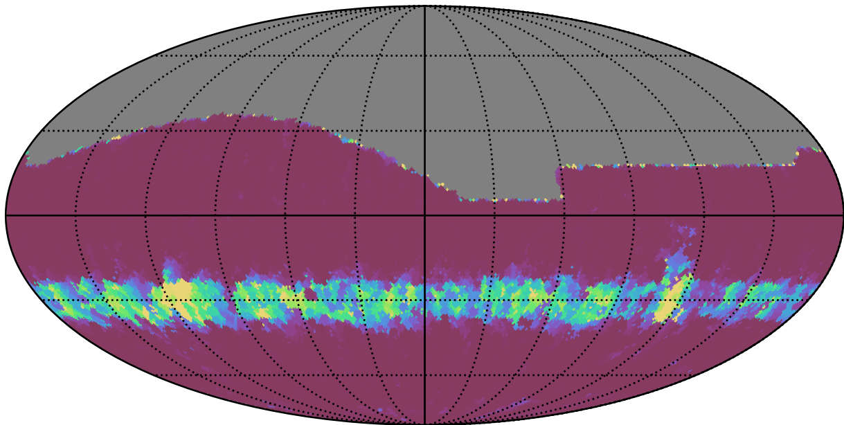
baseline_v3.0_10yrs All sky g band: Min normairmass
