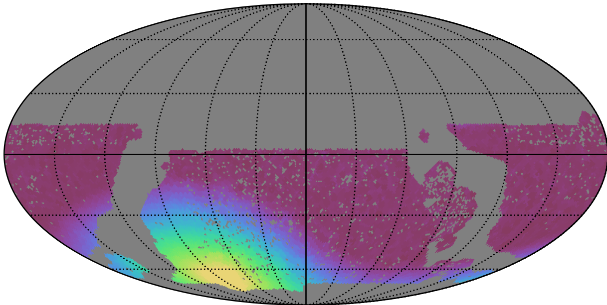
baseline_v3.0_10yrs WFD z band: Min moonDistance
