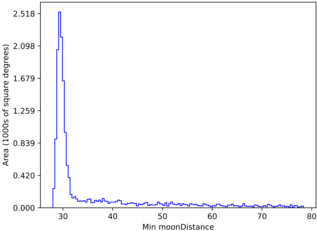
baseline_v3.0_10yrs WFD z band: Min moonDistance
