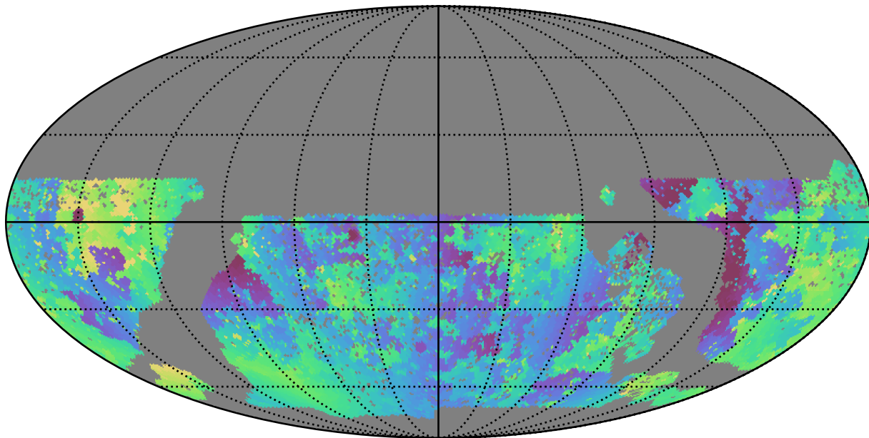
baseline_v3.0_10yrs WFD u band: Min moonDistance
