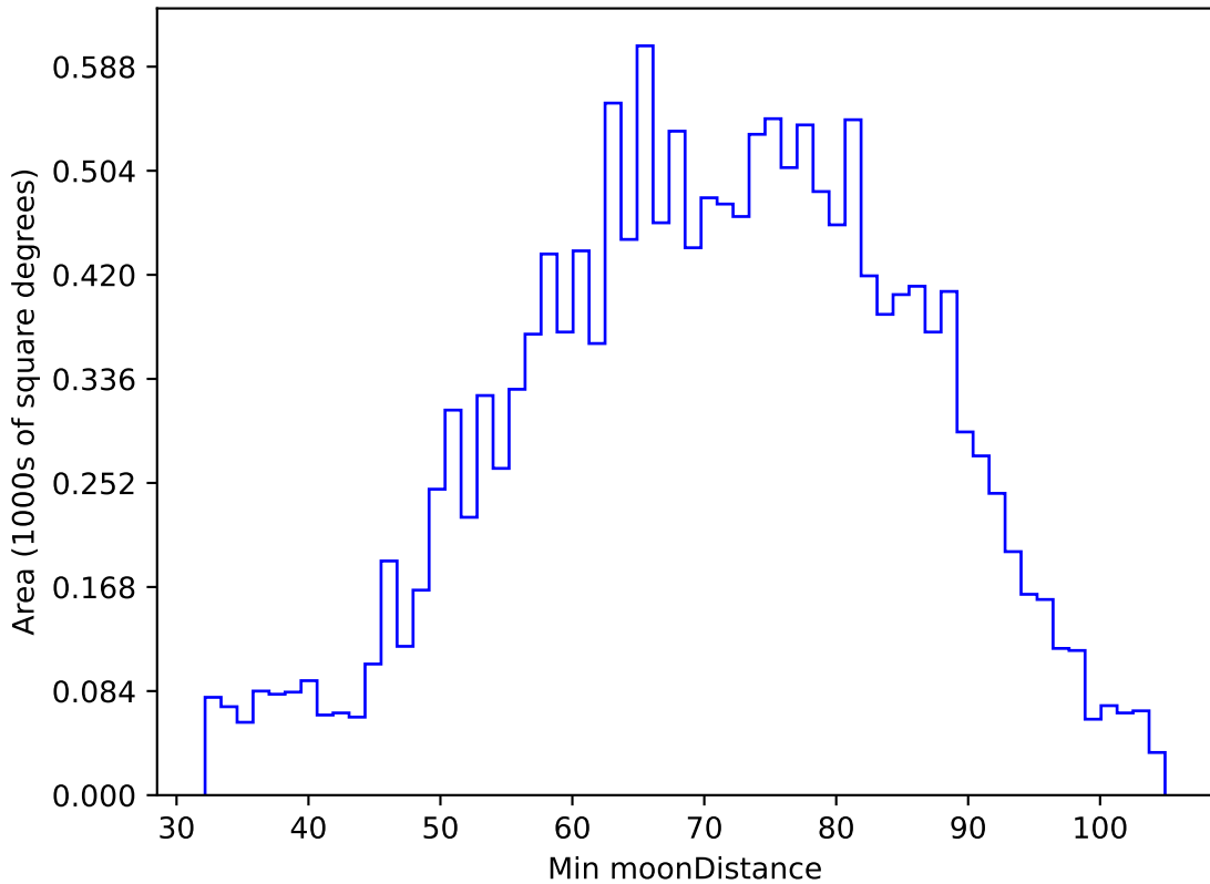
baseline_v3.0_10yrs WFD u band: Min moonDistance
