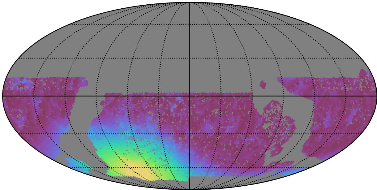
baseline_v3.0_10yrs WFD r band: Min moonDistance
