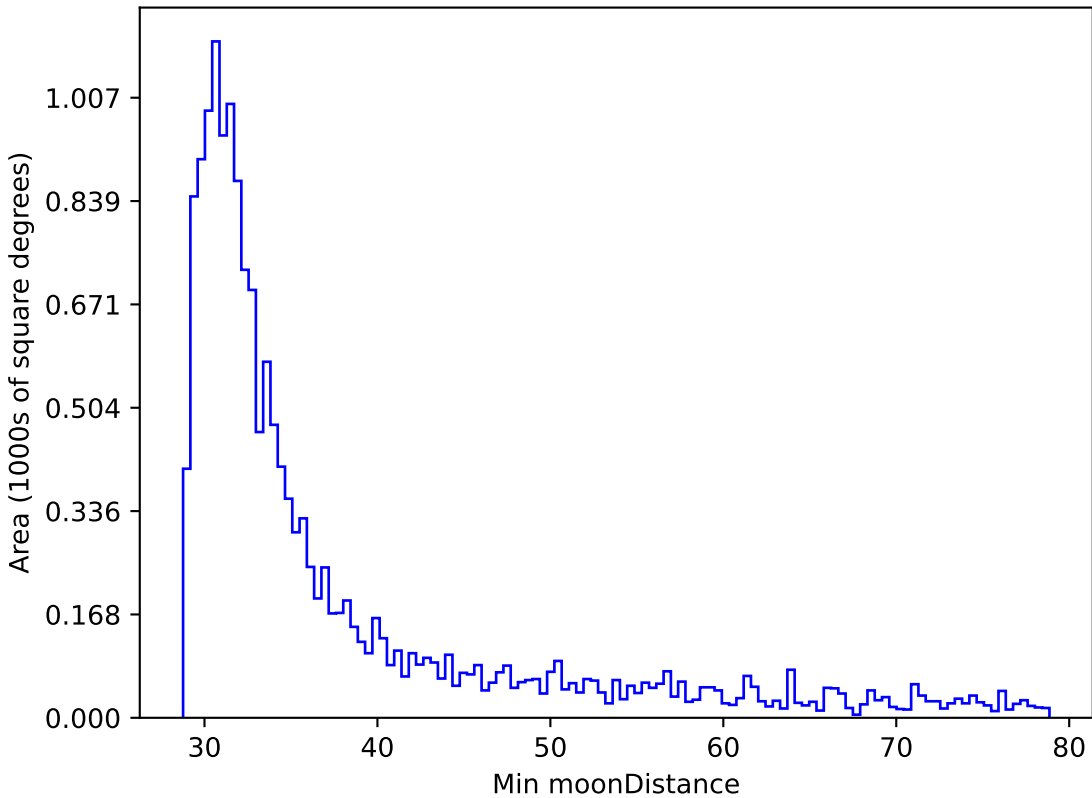
baseline_v3.0_10yrs WFD r band: Min moonDistance
