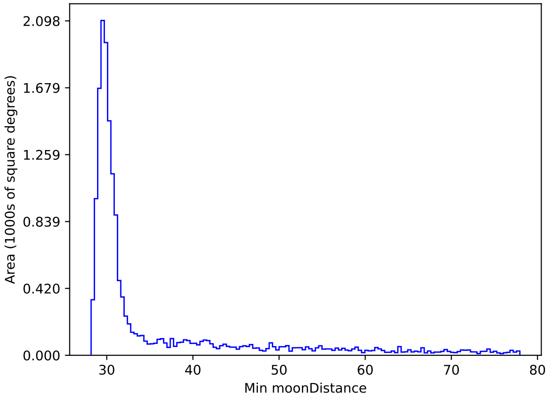
baseline_v3.0_10yrs WFD i band: Min moonDistance
