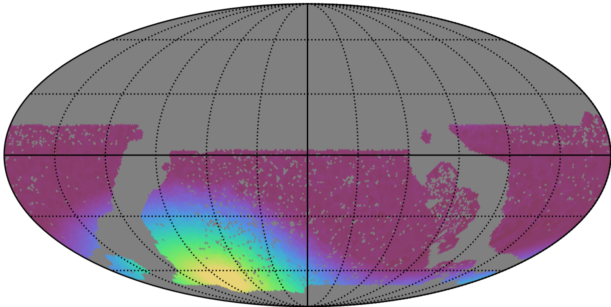
baseline_v3.0_10yrs WFD all bands: Min moonDistance
