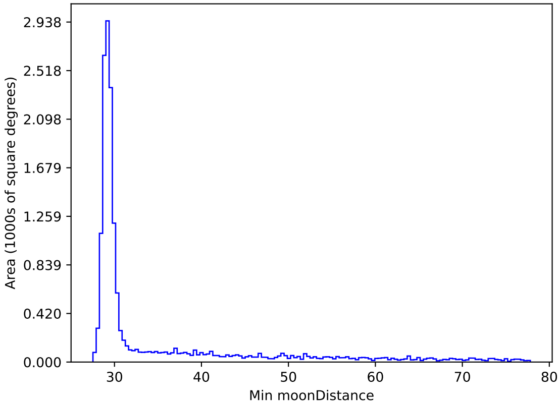
baseline_v3.0_10yrs WFD all bands: Min moonDistance
