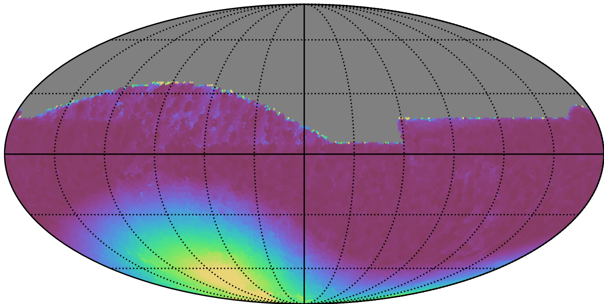
baseline_v3.0_10yrs All sky z band: Min moonDistance
