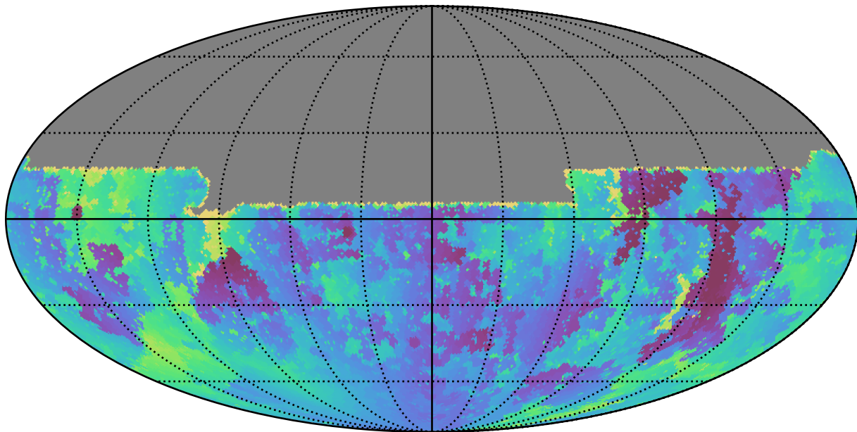
baseline_v3.0_10yrs All sky u band: Min moonDistance
