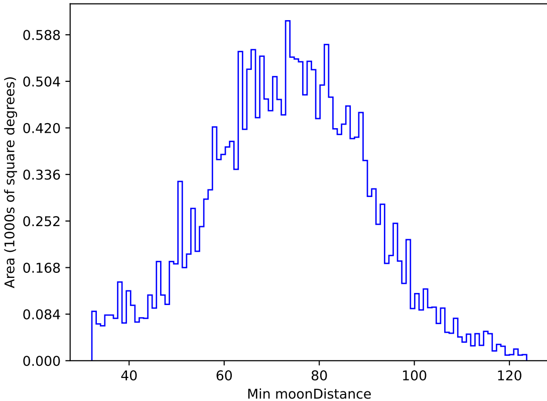
baseline_v3.0_10yrs All sky u band: Min moonDistance
