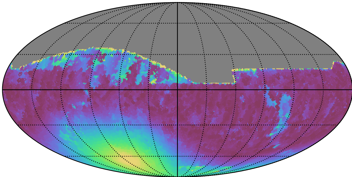
baseline_v3.0_10yrs All sky r band: Min moonDistance
