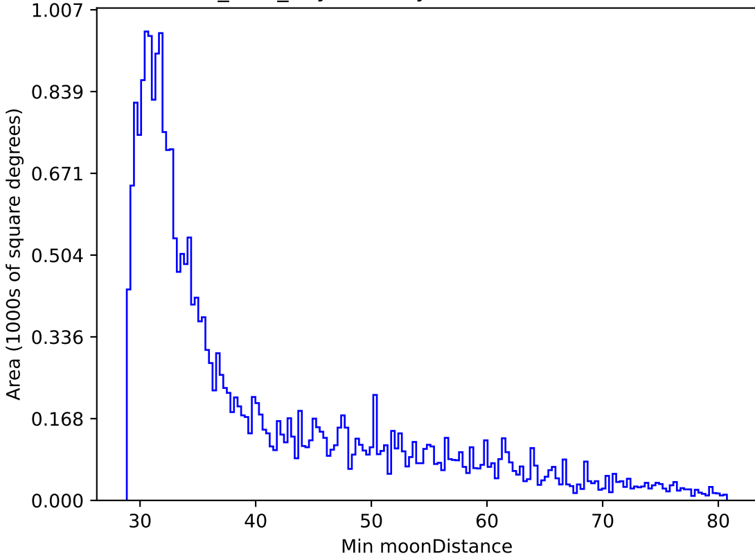
baseline_v3.0_10yrs All sky r band: Min moonDistance
