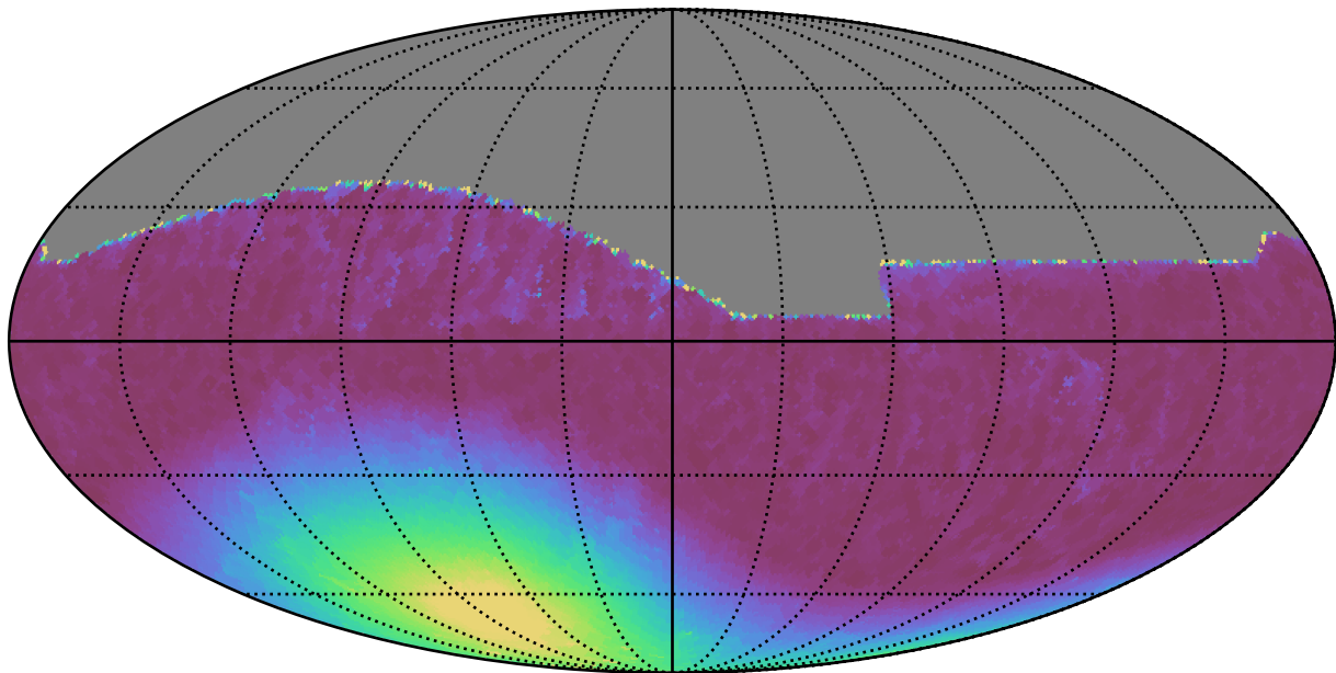
baseline_v3.0_10yrs All sky i band: Min moonDistance
