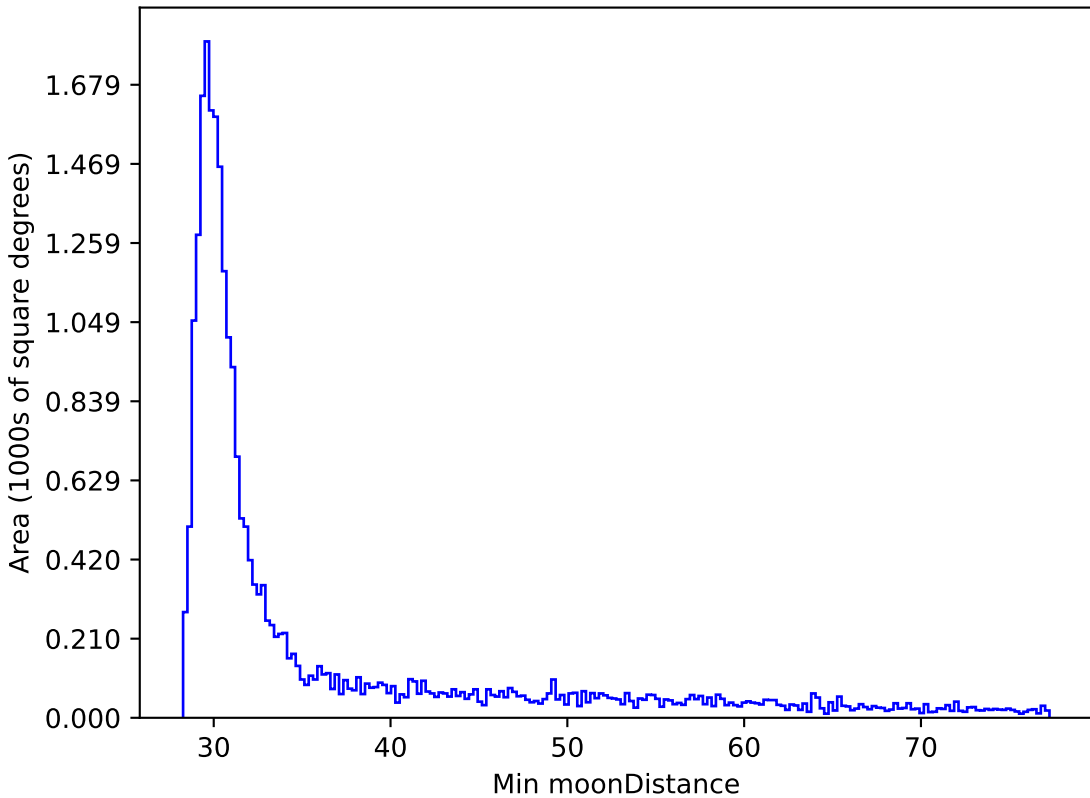
baseline_v3.0_10yrs All sky i band: Min moonDistance
