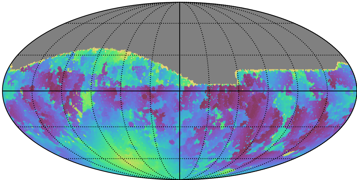
baseline_v3.0_10yrs All sky g band: Min moonDistance
