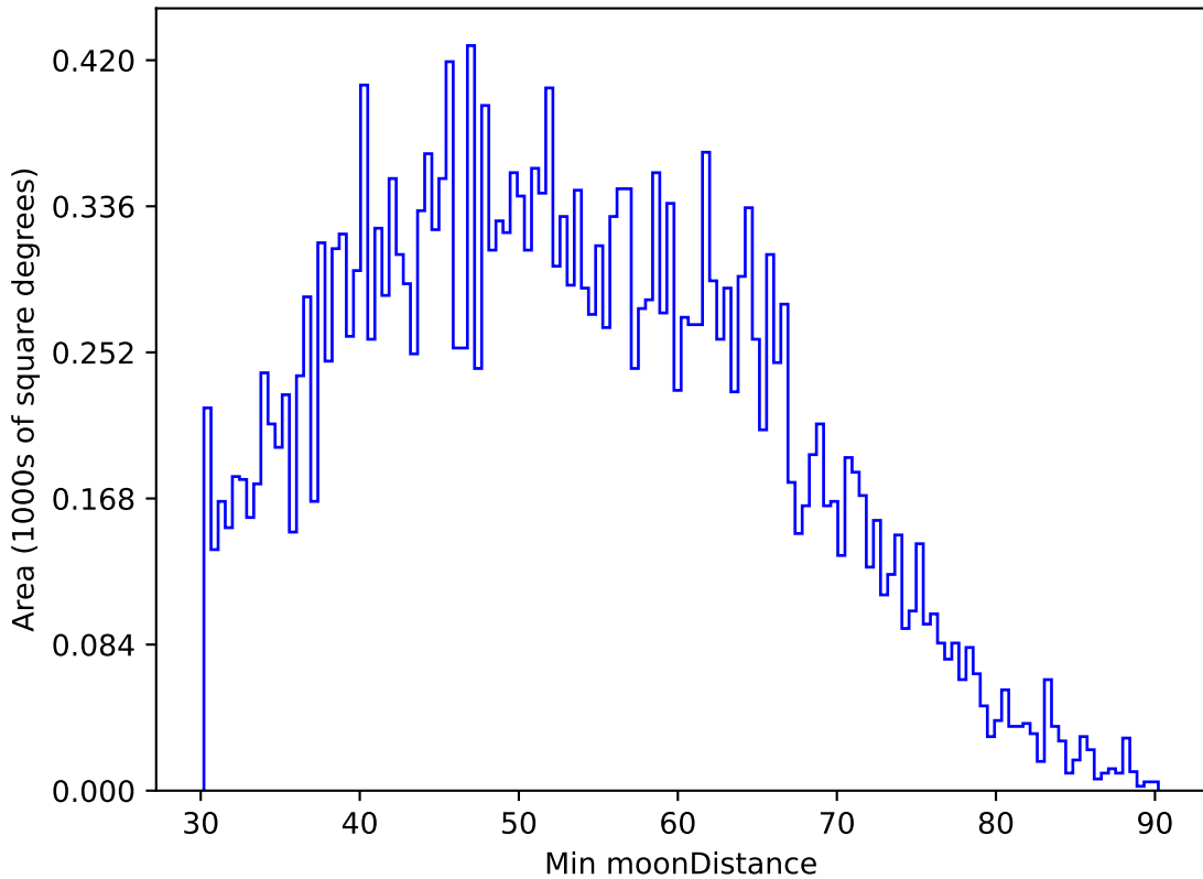
baseline_v3.0_10yrs All sky g band: Min moonDistance
