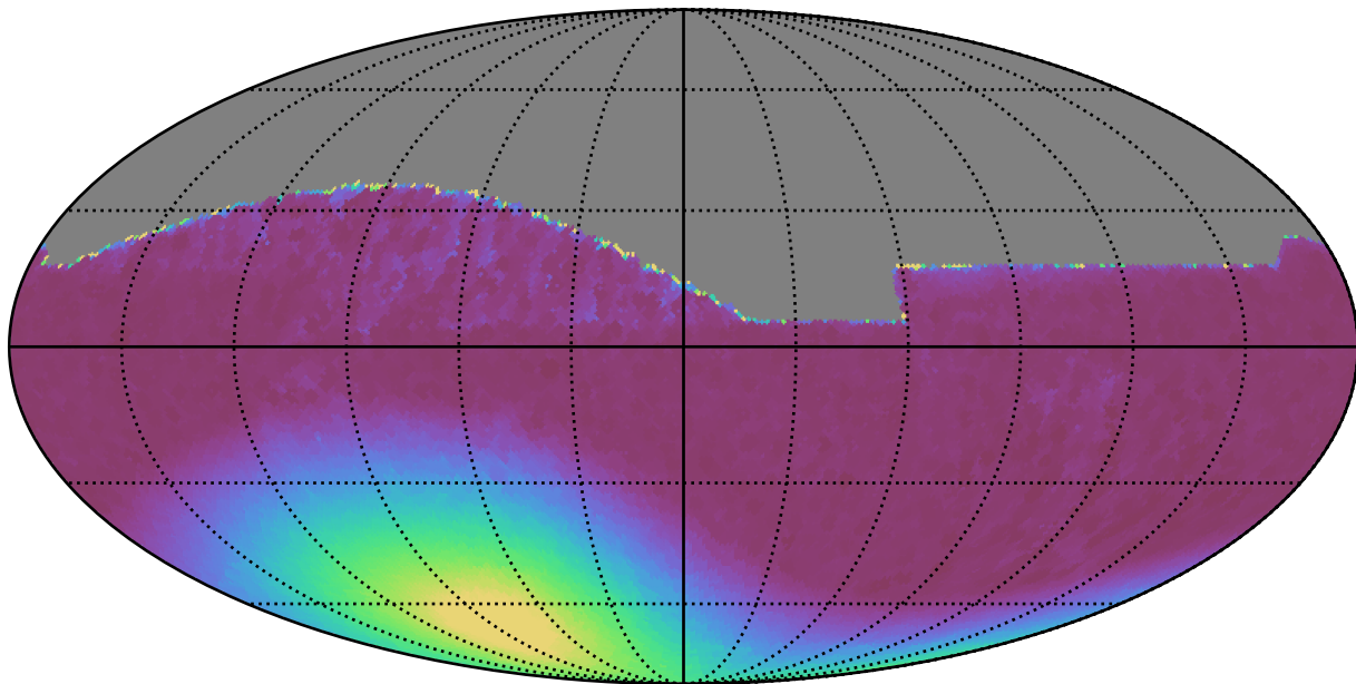
baseline_v3.0_10yrs All sky all bands: Min moonDistance
