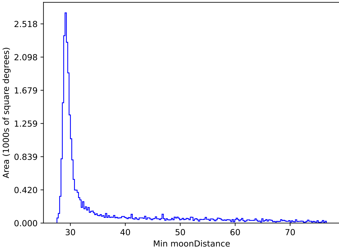
baseline_v3.0_10yrs All sky all bands: Min moonDistance
