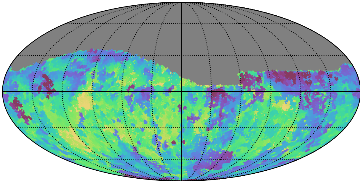
baseline_v3.0_10yrs Yr 1 z band: Min fiveSigmaDepth
