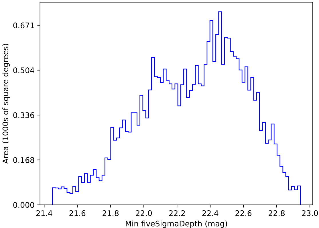
baseline_v3.0_10yrs Yr 1 z band: Min fiveSigmaDepth
