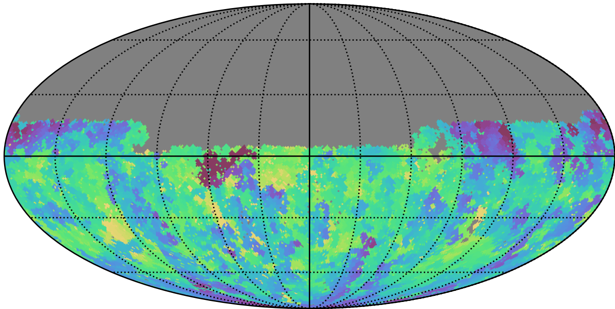
baseline_v3.0_10yrs Yr 1 u band: Min fiveSigmaDepth
