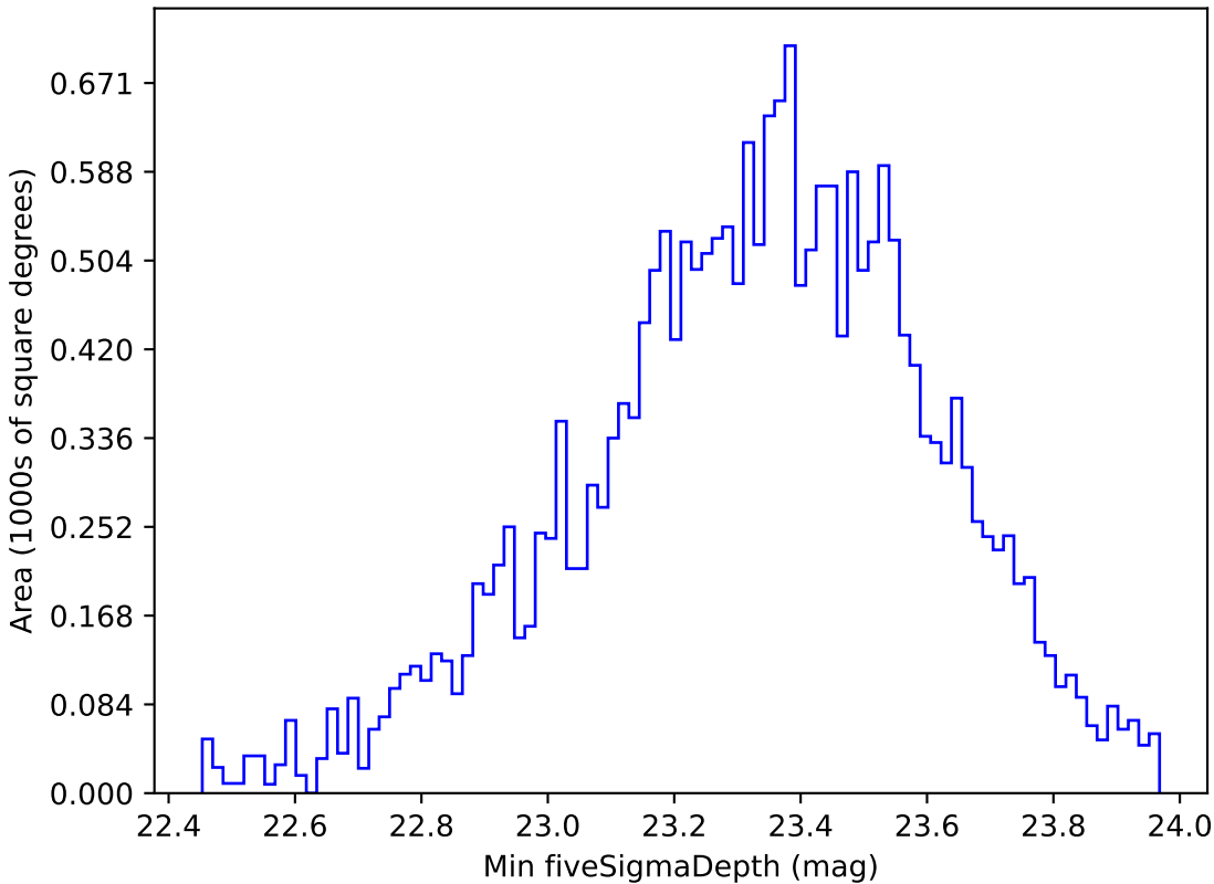
baseline_v3.0_10yrs Yr 1 u band: Min fiveSigmaDepth
