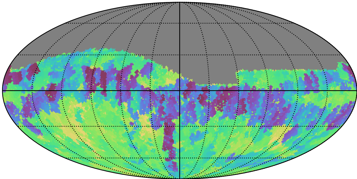
baseline_v3.0_10yrs Yr 1 r band: Min fiveSigmaDepth
