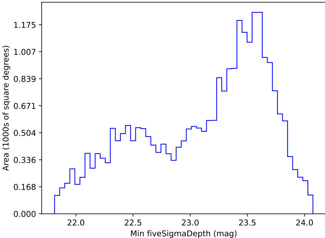
baseline_v3.0_10yrs Yr 1 r band: Min fiveSigmaDepth
