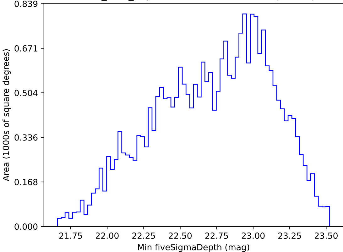
baseline_v3.0_10yrs Yr 1 i band: Min fiveSigmaDepth
